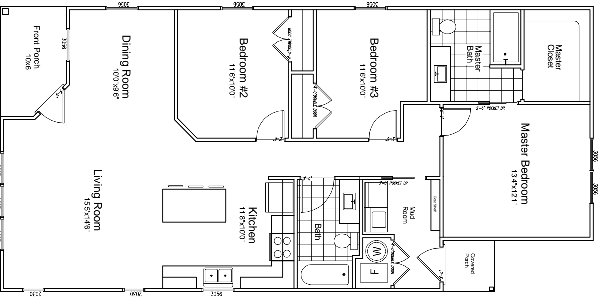
First Floor Plan 26' x 54'
